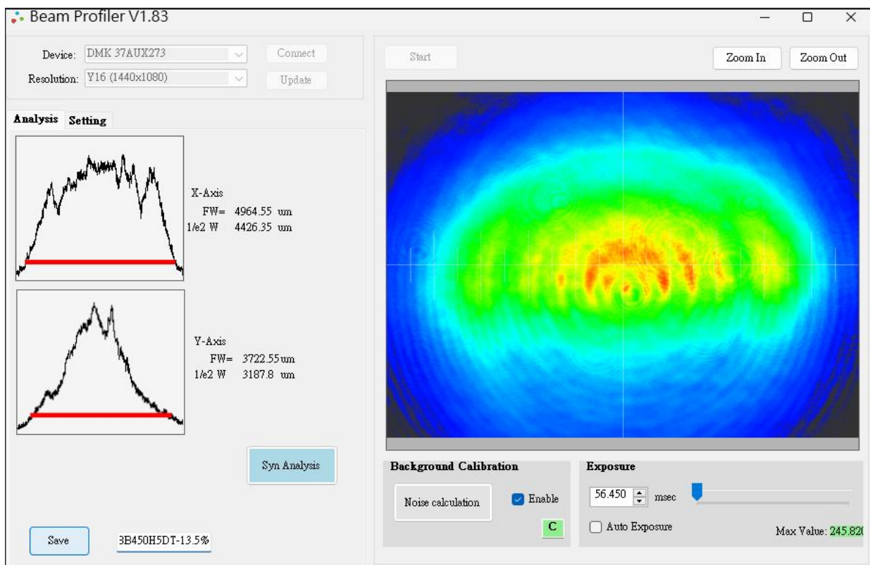
LM8 series Blue Dot Profile at 1m
