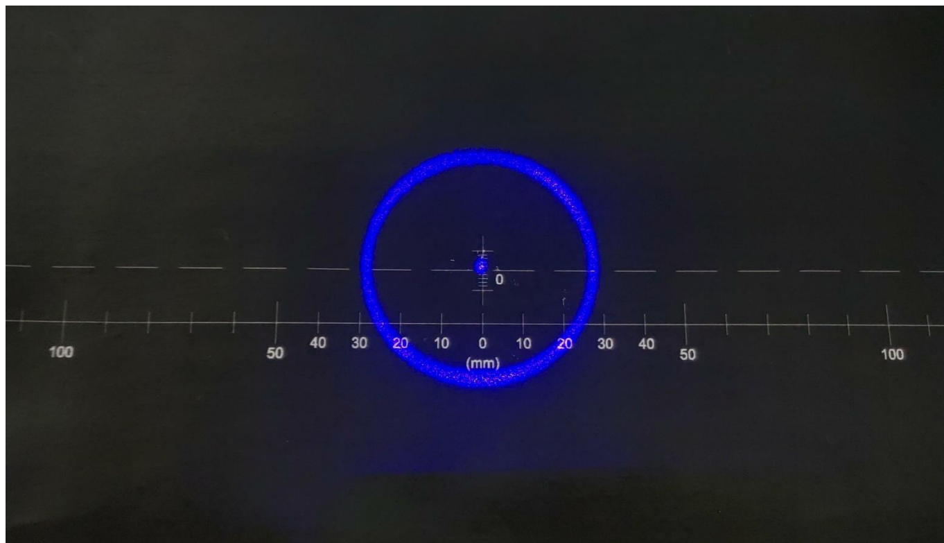
LM9B450S5P37 Beam Shape at 1m
