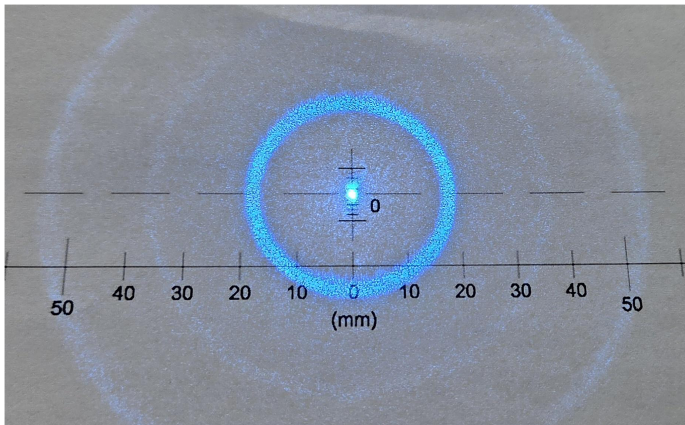
LM9B490H10P39 Beam Shape at 1m
