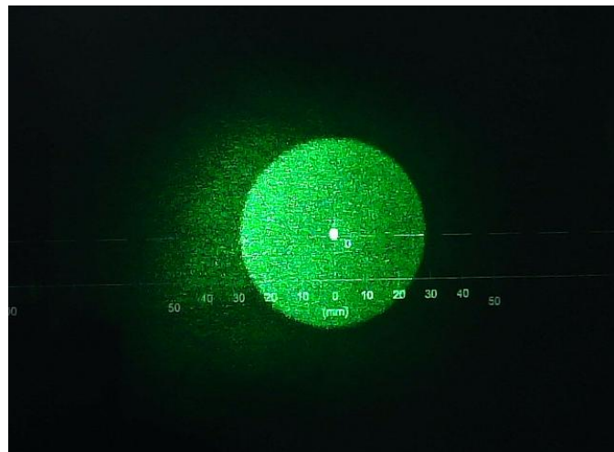
LM9G520H30P2 Beam Shape at 50cm
