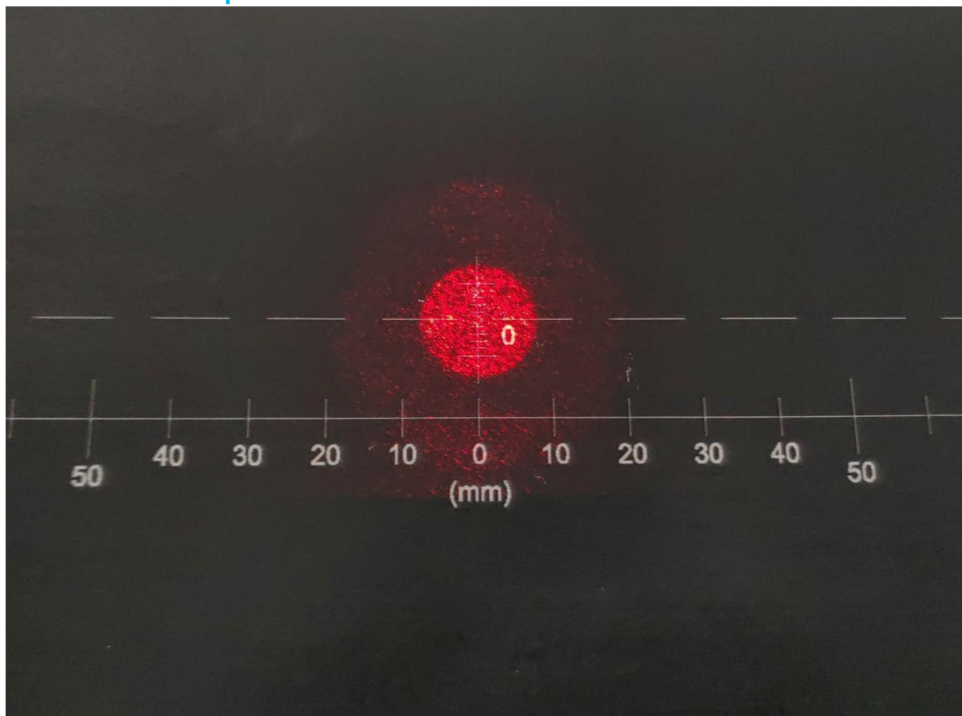
LM9R635H10P4 Beam Shape at 1m
