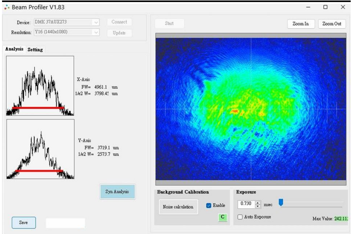
LM8IR830H200D beam profile data @1m
