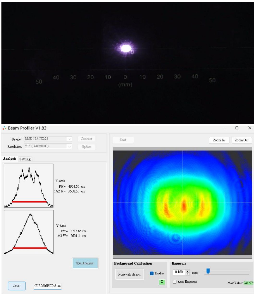
LM8IR980H50D Dot Shape at 1m
