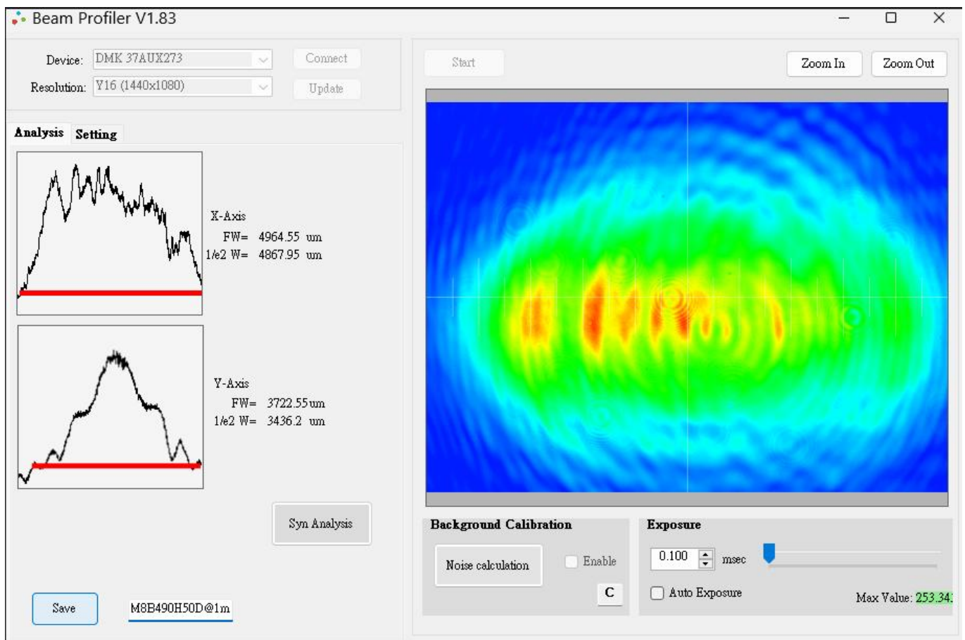
LM8 series Blue Dot Profile at 1m
